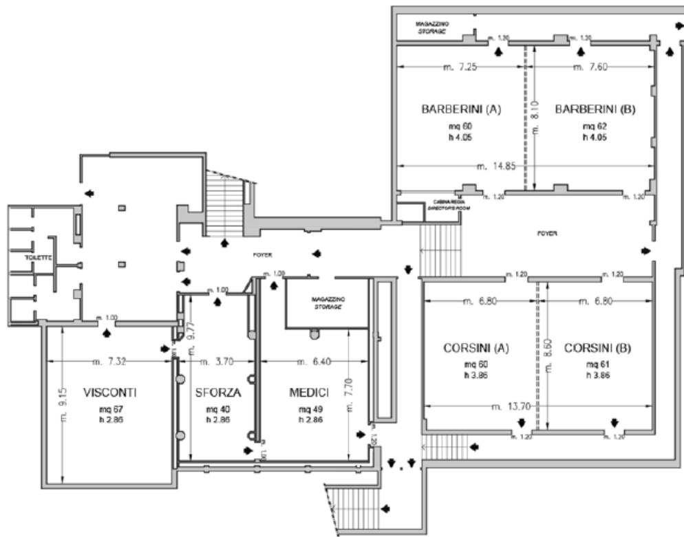
Piano -1 / Basement
