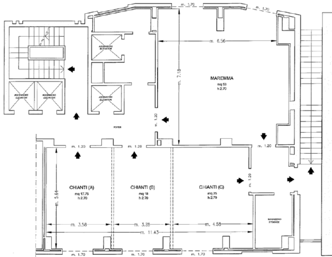
Piano Primo / First Floor
